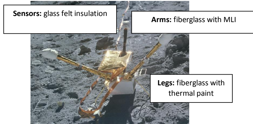
Figure B4 – Lunar Surface Magnetometer
