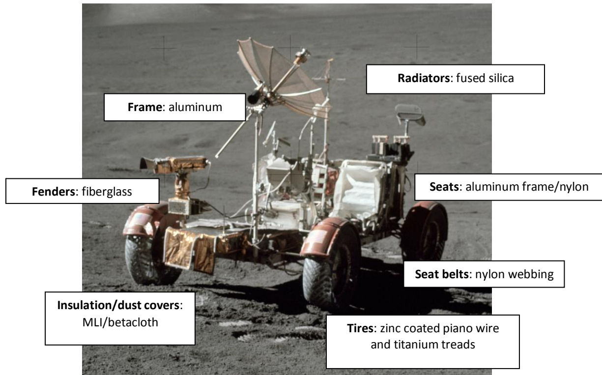
Figure B13 – Lunar Roving Vehicle
