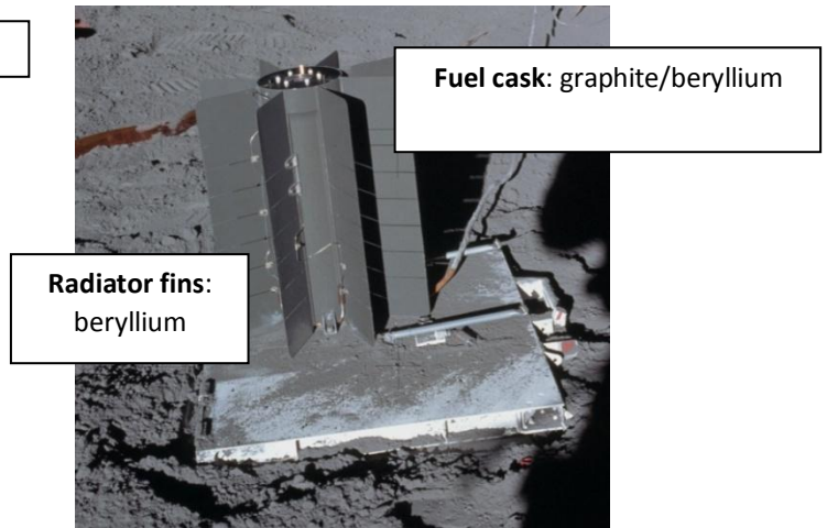
Figure B2 – RTG
