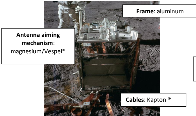
Figure B1 – ALSEP Central Station
