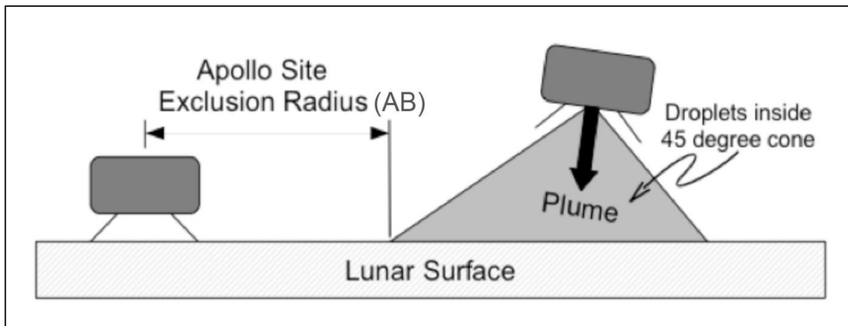
Figure 12: Illustration of plume droplet cone.
