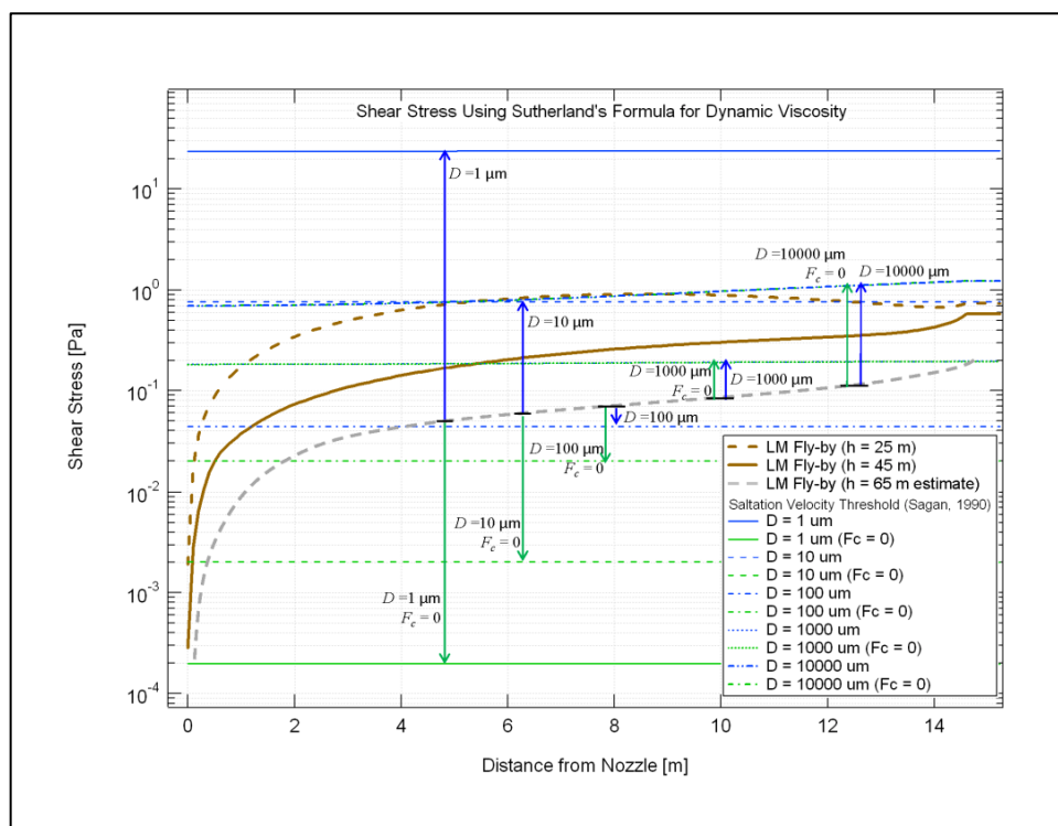
Figure 11: Shear stress generated by a rocket exhaust plume and shear stress levels required to mobilize various sizes of lunar soil particles.
