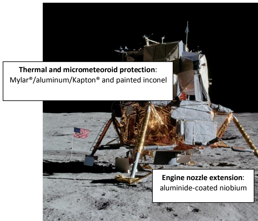
Figure B14 – Lunar Module Descent Stage (Shown with Ascent Stage)
