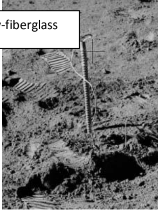
Figure B7 – Heat Flow Experiment
