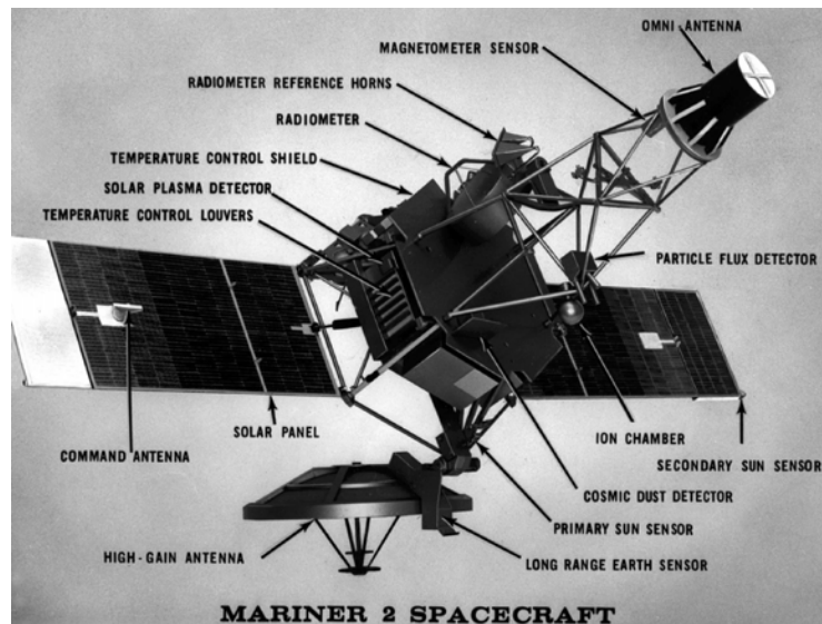
The Mariner 2 spacecraft. Note that the solar arrays are not the same size. The panel on the right side of the image is longer than that of the left; the white tip on the left panel was a cloth extension designed to even out the solar wind pressure on the spacecraft.
